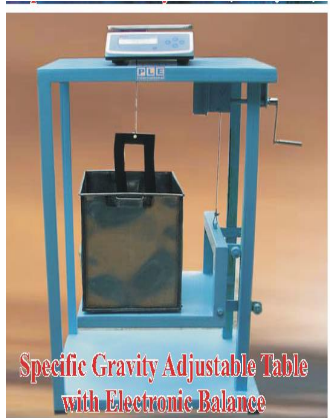
Product# 03-160 Specific Gravity Table
